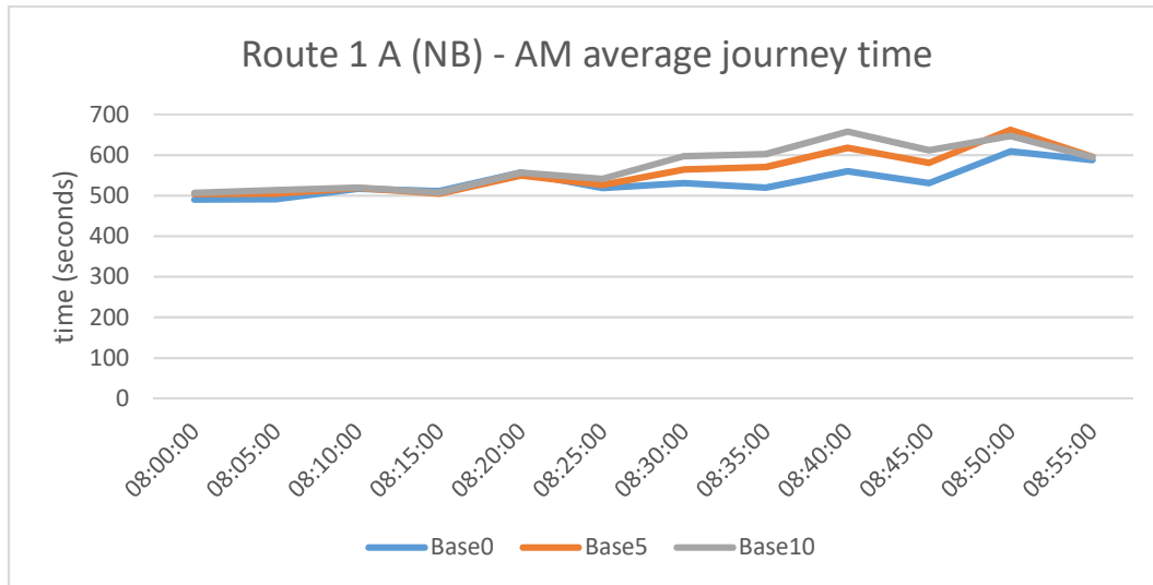
Figure 3.46 - Route 1A - AM average journey time
