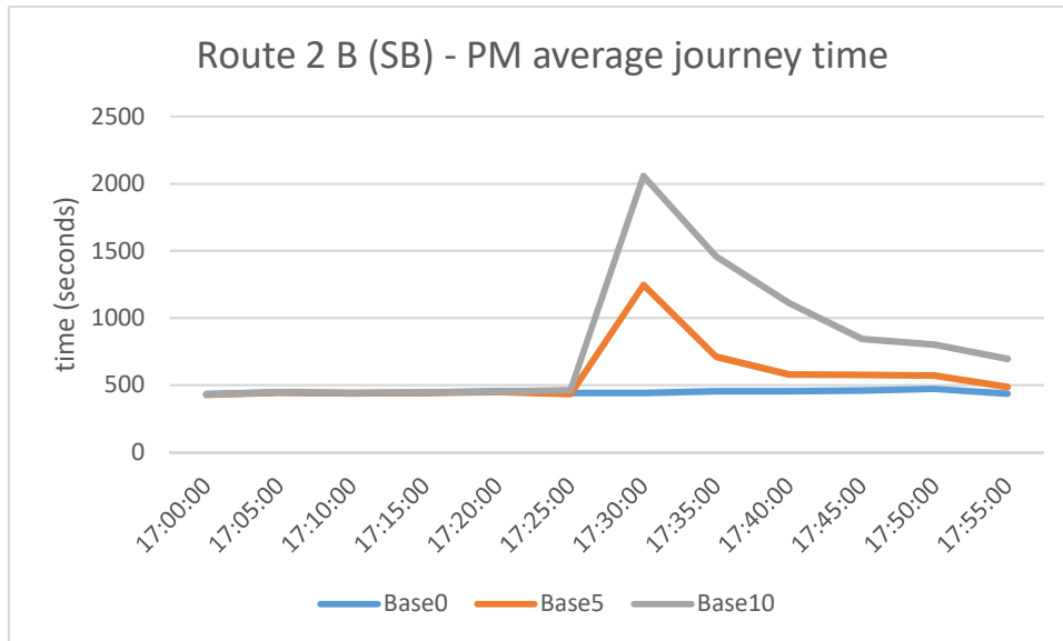
Figure 3.57 - Route 2B - PM average journey time
