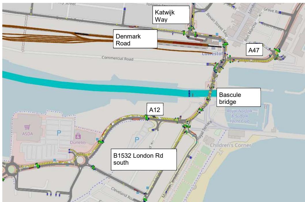
Figure 3.28 – Base AM Peak Bascule Bridge (5 min lift - 08:36 after reopening to vehicular traffic)
