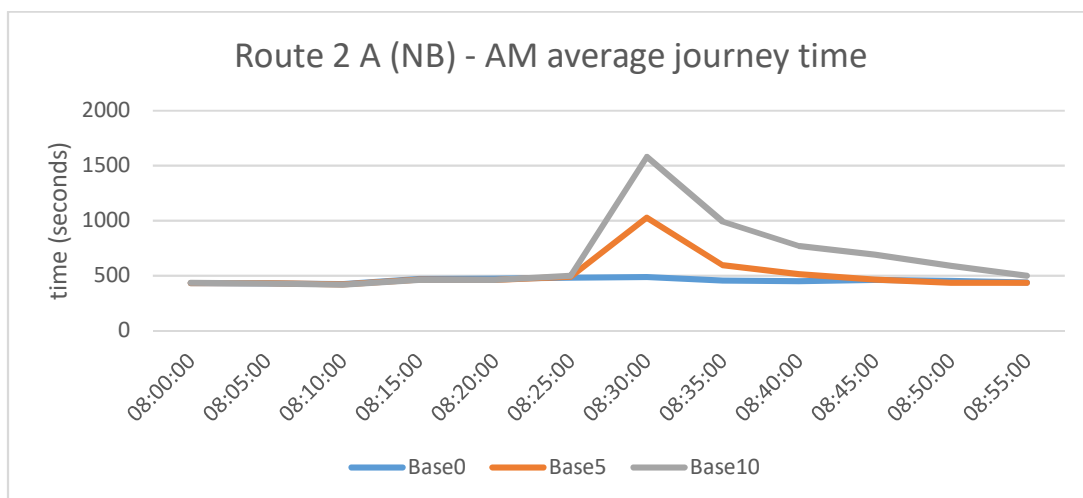
Figure 3.48 - Route 2A - AM average journey time
