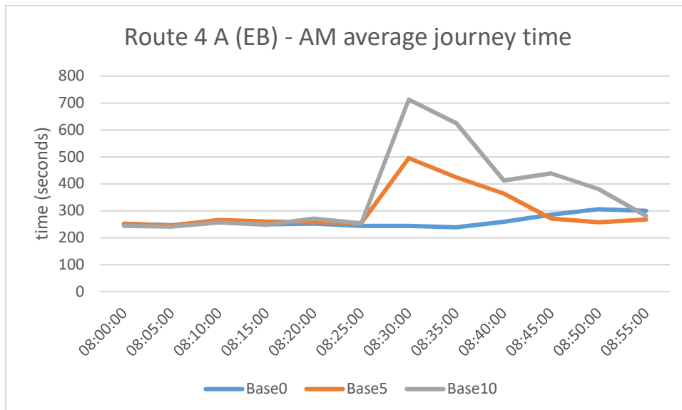
Figure 3.52 - Route 4A - AM average journey time
