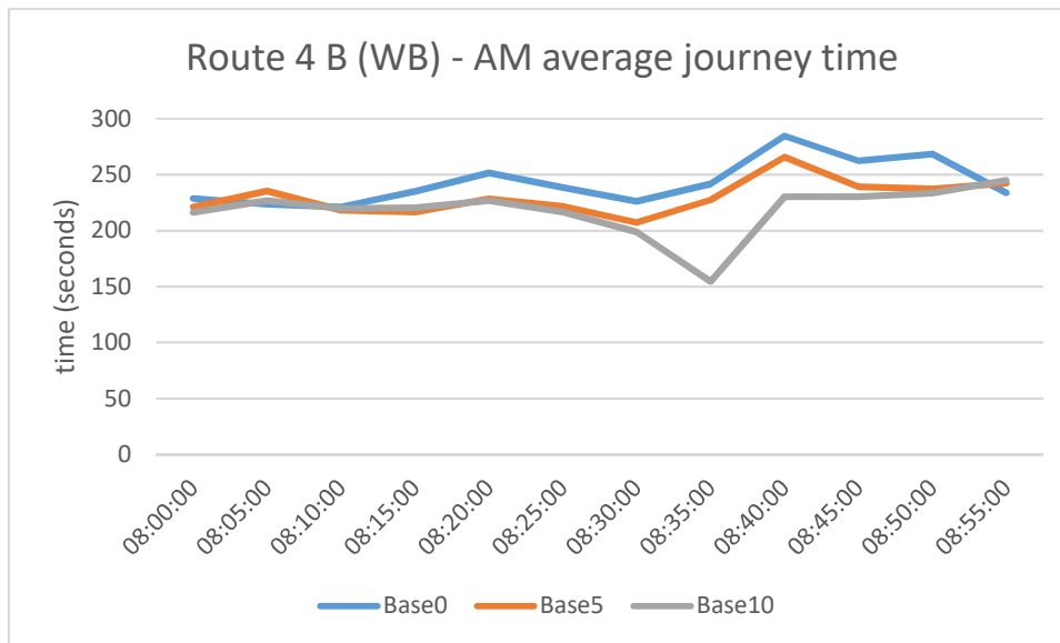
Figure 3.53 - Route 4B - AM average journey time
