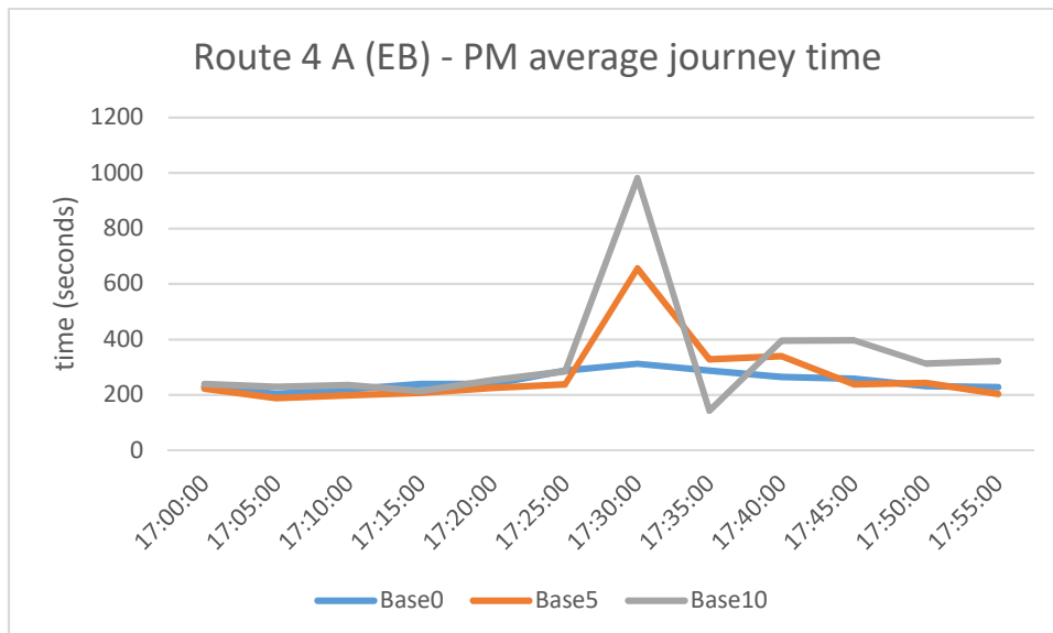
Figure 3.60 - Route 4A - PM average journey time
